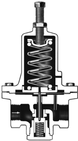
TYPE 95H OR 95HT REGULATOR WITH METAL DIAPHRAGM AND METAL SEATING SURFACES
