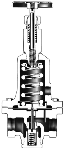
TYPE 95HD REGULATOR WITH METAL DIAPHRAGM AND SEAT, ALSO TYPICAL OF TYPE 95LD
