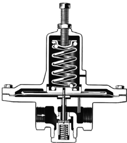
TYPE 95L REGULATOR WITH NEOPRENE DIAPHRAGM AND NEOPRENE VALVE DISK
