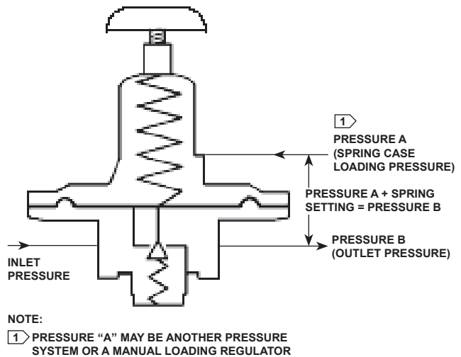
Figure 4. Operational Schematic for Types 95LD and 95HD Regulators
