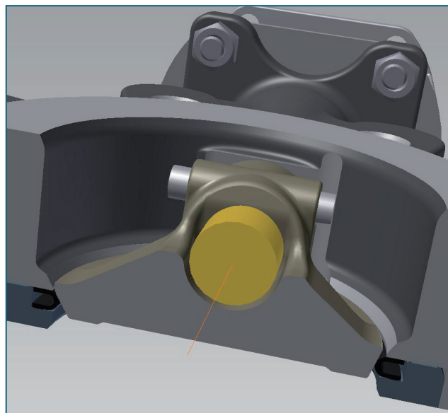
The sealing system of the CV 300.
